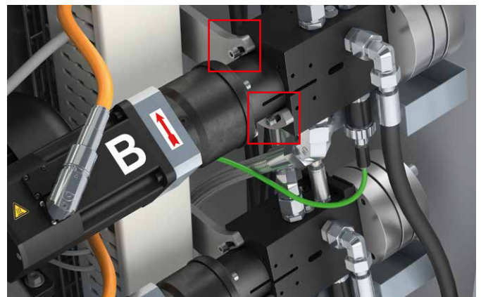
In order to remove the pump including the drive train, only 2 screws need to be loosened.
