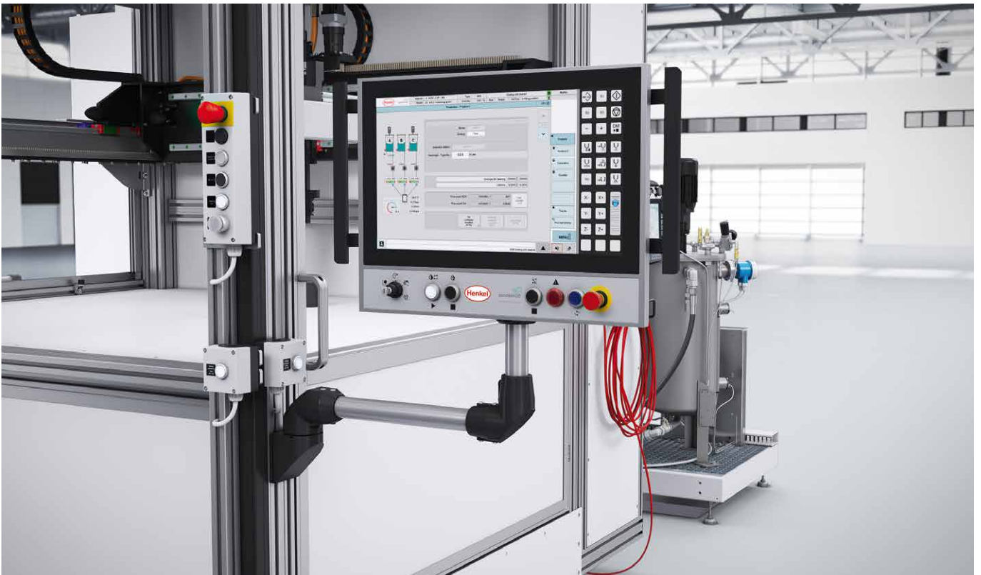
Optional: CONTROL 2 multi-touch operating panel, mounted laterally on a swivel arm, with display elements and operating keys, visualization via 21.5" touchscreen. With this option, you also receive the multi-function MP 2 mobile panel.
