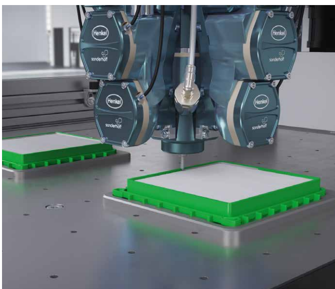
FERMAPOR adhesive sealant dosed application with the MK 800 PRO mixing head for bonding the filter pack into the frame
