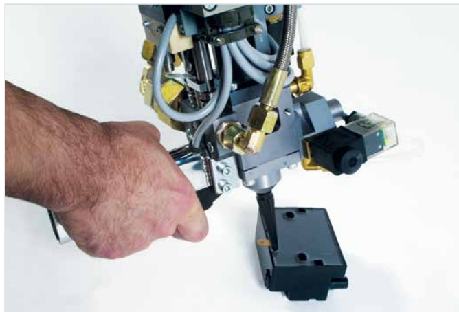
Manual potting of an electronic component with the MK 50 mixing head and the 2-component casting resin FERMADUR from Henkel
