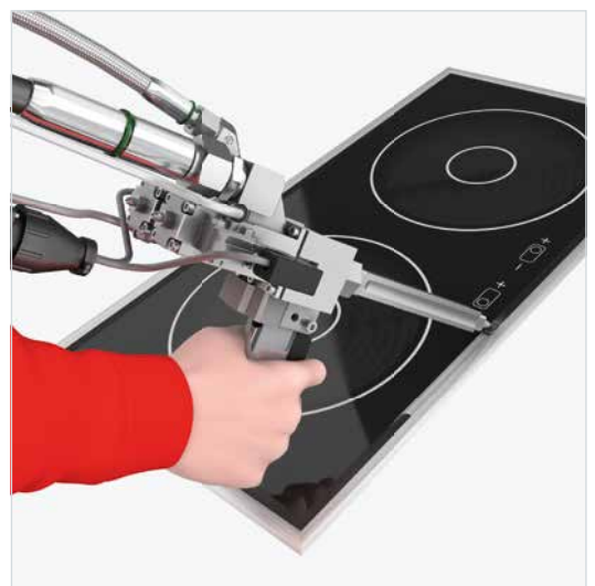
Manual potting with the MK 20/21 mixing head
