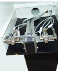
Primer application unit – the optional primer nozzle mounted on the rear of the CNC Y-axis applies the primer in parallel to the seal application on powder-coated or stainless steel surfaces in the same contour.
